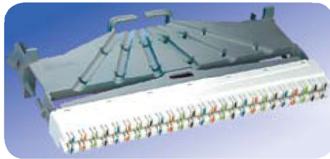
HighBand® 25 block rear cable manager
