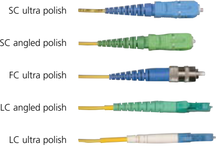
Connector Types
