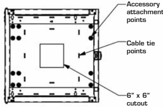
Rear Panel View (Interior Detail)
