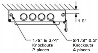
Rear Panel View (Top/Bottom Detail)
