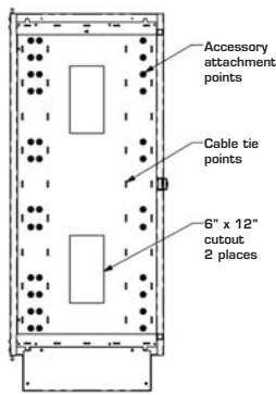
Rear Panel View (Interior Detail)
