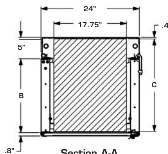
Section A-A (Interior Detail)
