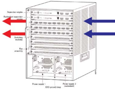
Figure 4 – Cisco switch side-to-side airflow
