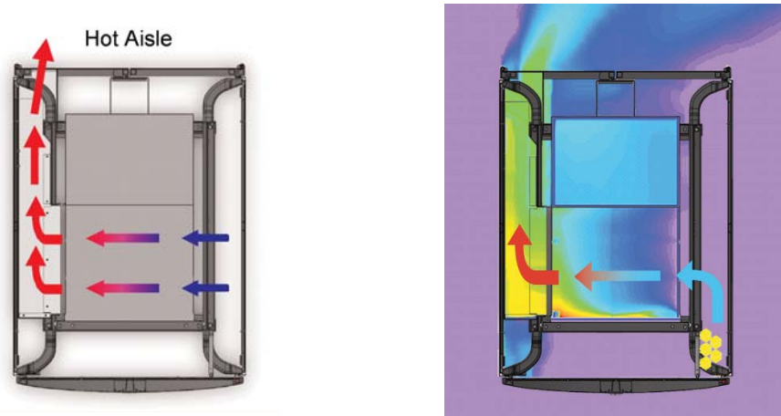
Figure 6 – Re-directing exhaust out rear of cabinet
